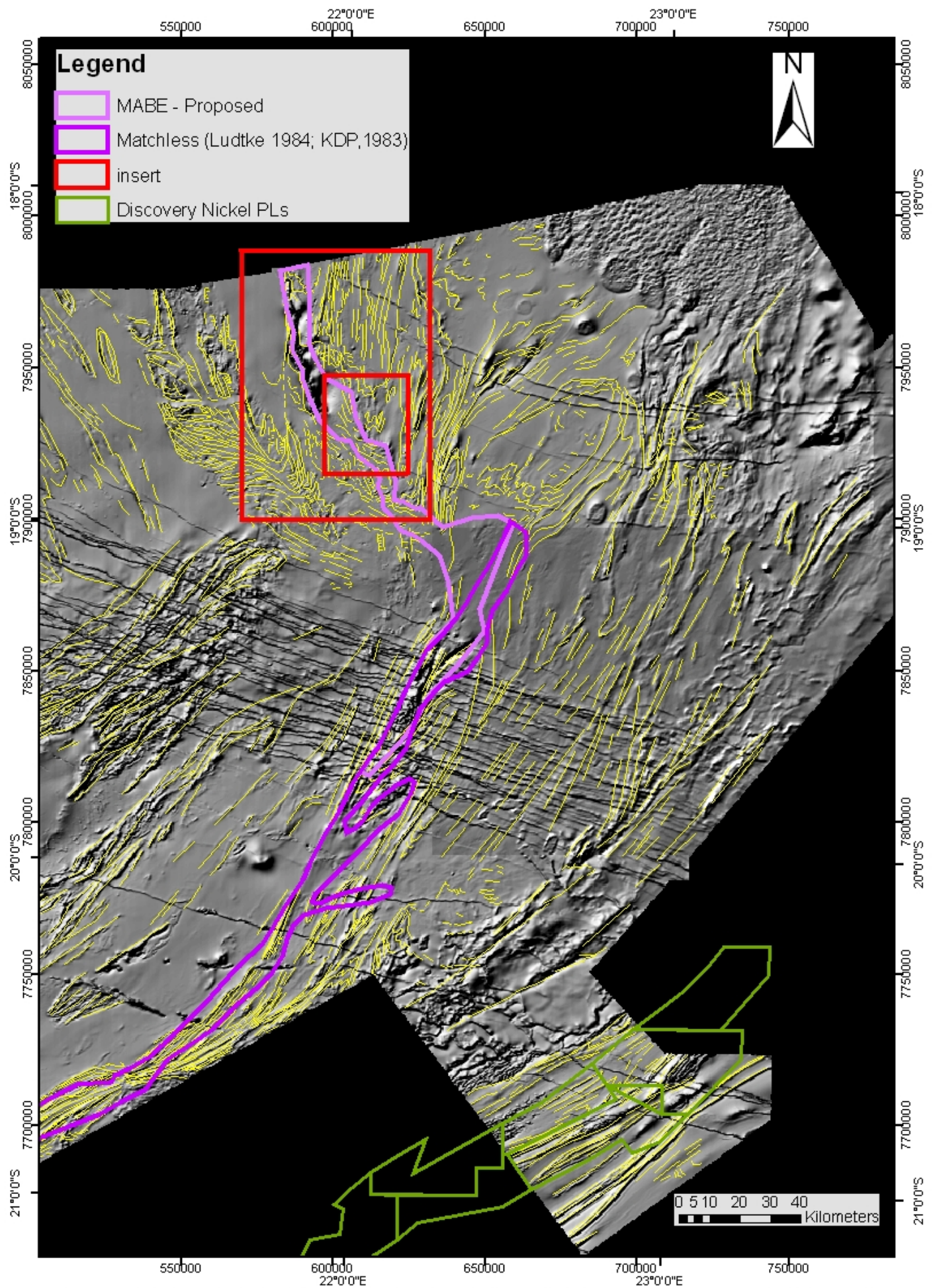
Figure 5 Hillshaded aeromagnetic data image overlain by lithotectonic trends in the Pan African Basement. The Matchless Amphibolite Belt Extension (MABE) as proposed in this study is shown. The inserts show the location of figures 7 - 10.
