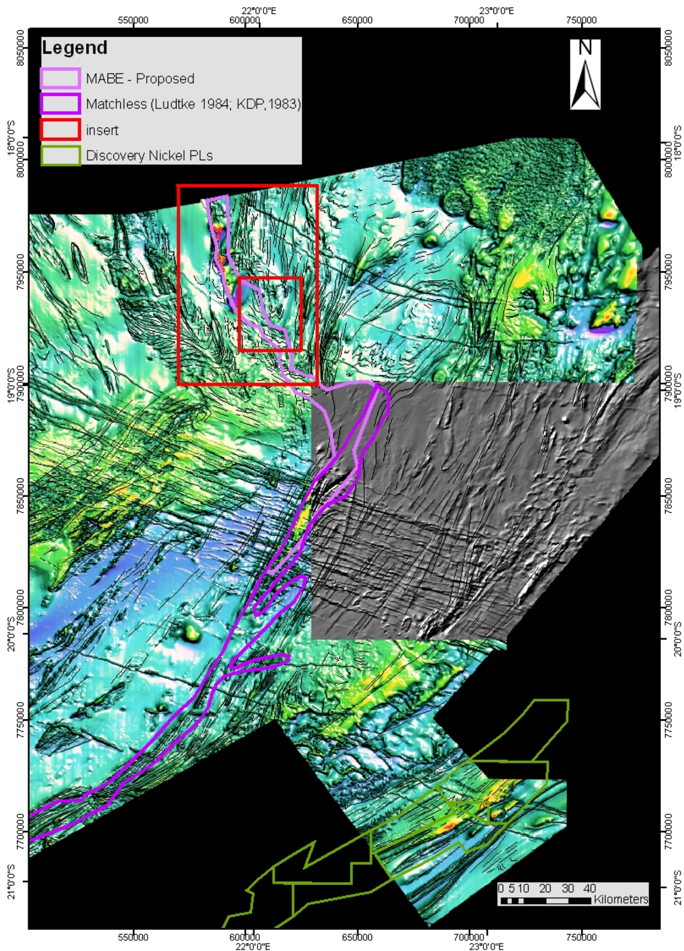
Figure 6 Structurally enhanced aeromagnetic data image overlain by lithotectonic trends in the Pan African Basement. (Hillshaded image shown where enhanced imagery is unavailable.) The inserts show the location of figures 7 - 10.
